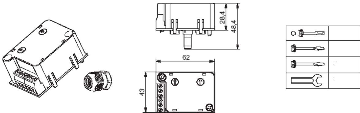
Abbildung 20: Modul 2 Signalschalter (SPDT), VA1000-S2 (in mm)
